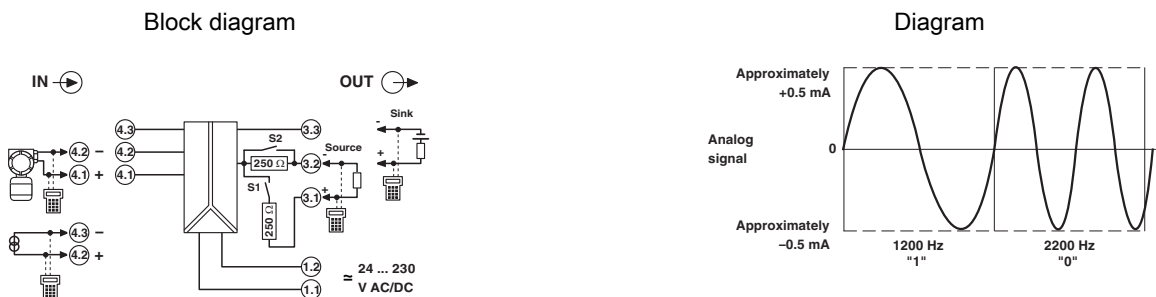
Signal transmission analog and digital at the same time
